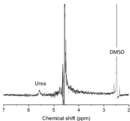
Supplementary Fig. 10 | 1 H NMR spectroscopy of Cu/Zn hybrid catalyst. We also detected the urea product by 1 H NMR spectroscopy. To suppressing water peak, we did not use D 2 O and used pure DMSO as the reference solution that was mixed with catholyte after electrolysis.
