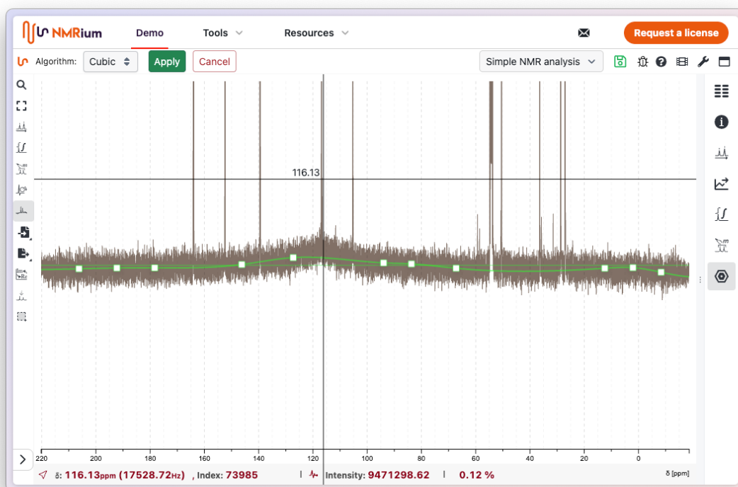
Baseline correction with movable anchors (source: docs.nmrium.org)
