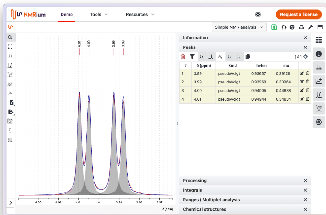
Fitting individual peak shapes by deconvolution (source: docs.nmrium.org)
